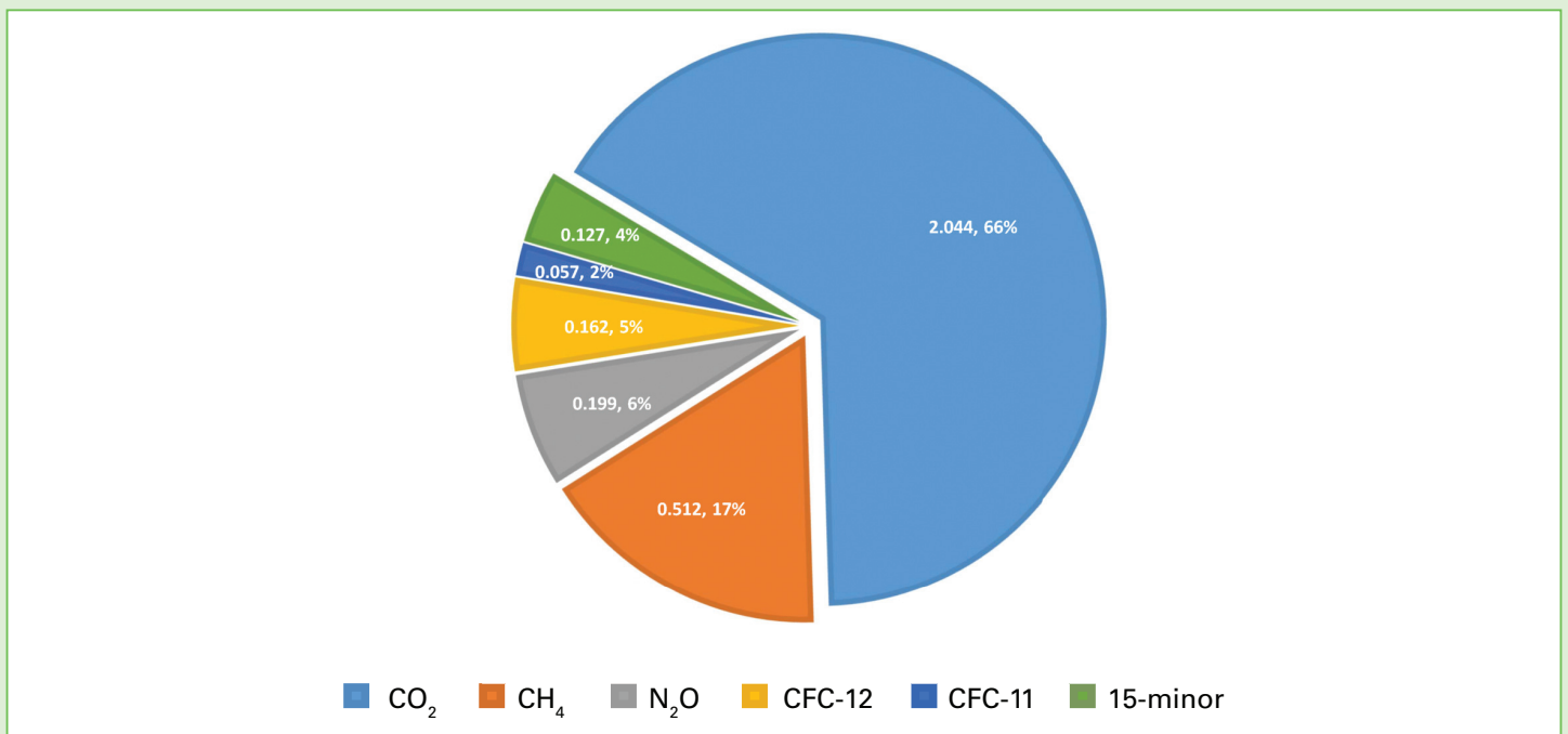
Figure 6. Increase in global radiative forcing in 2018 since pre-industrial times, resulting from an increase atmospheric burden of the most important LLGHGs, expressed in \text{W}\cdot\text{m}^{-2} and relative to the total increase from all greenhouse gases of 3.1 \text{ W}\cdot\text{m}^{-2} [9].
